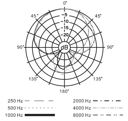
Q8 POLAR PATTERN
